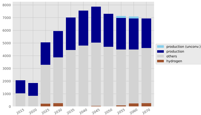
Gas supply (PJ)
