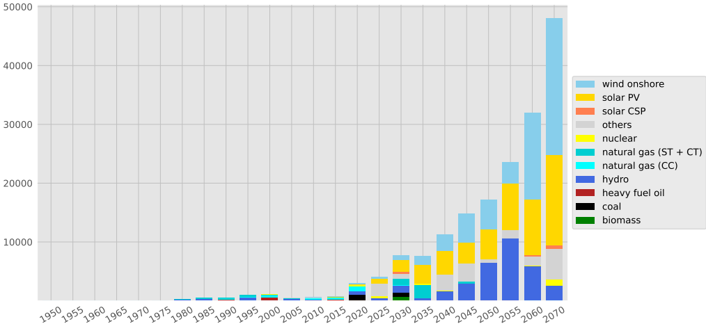
Power plant new capacity (MW)
